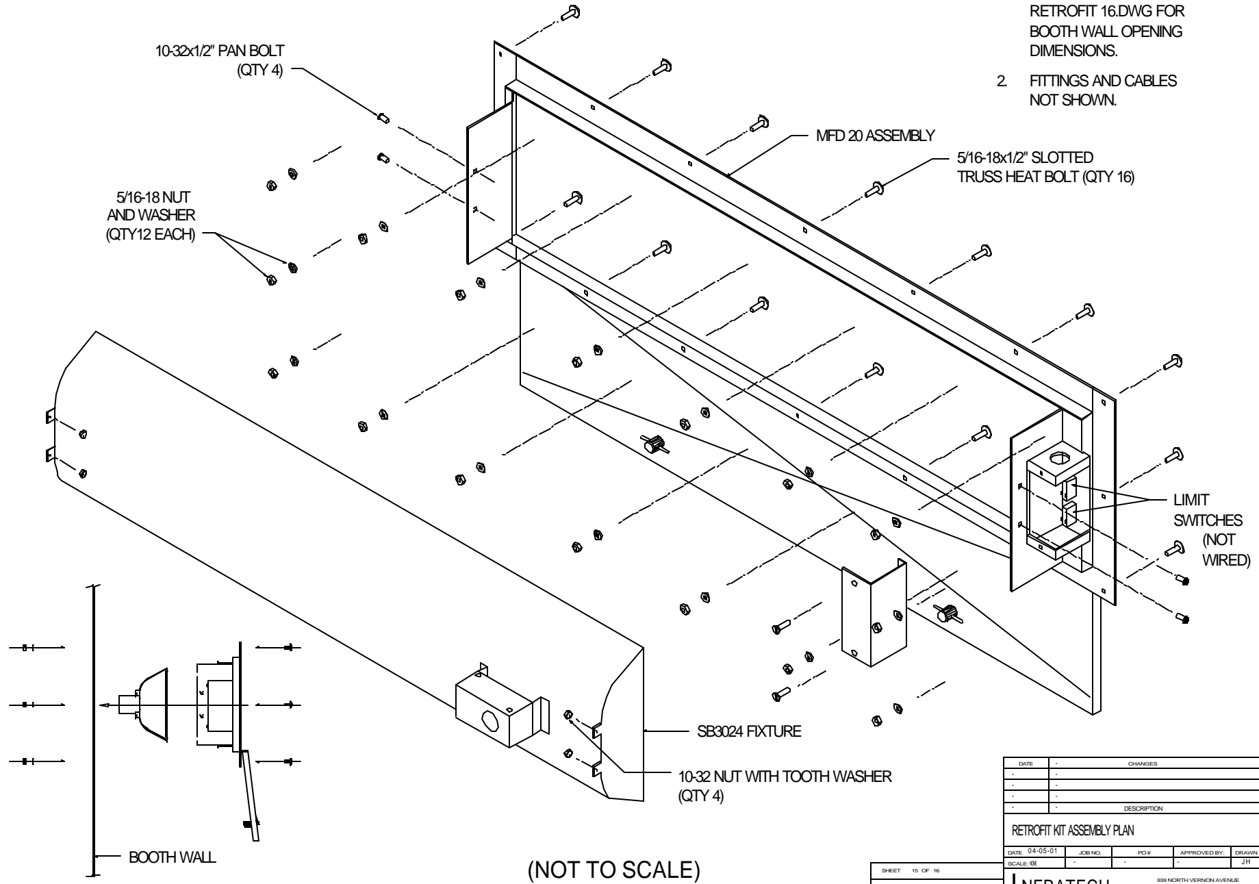
SIDE VIEW OF ASSEMBLY
